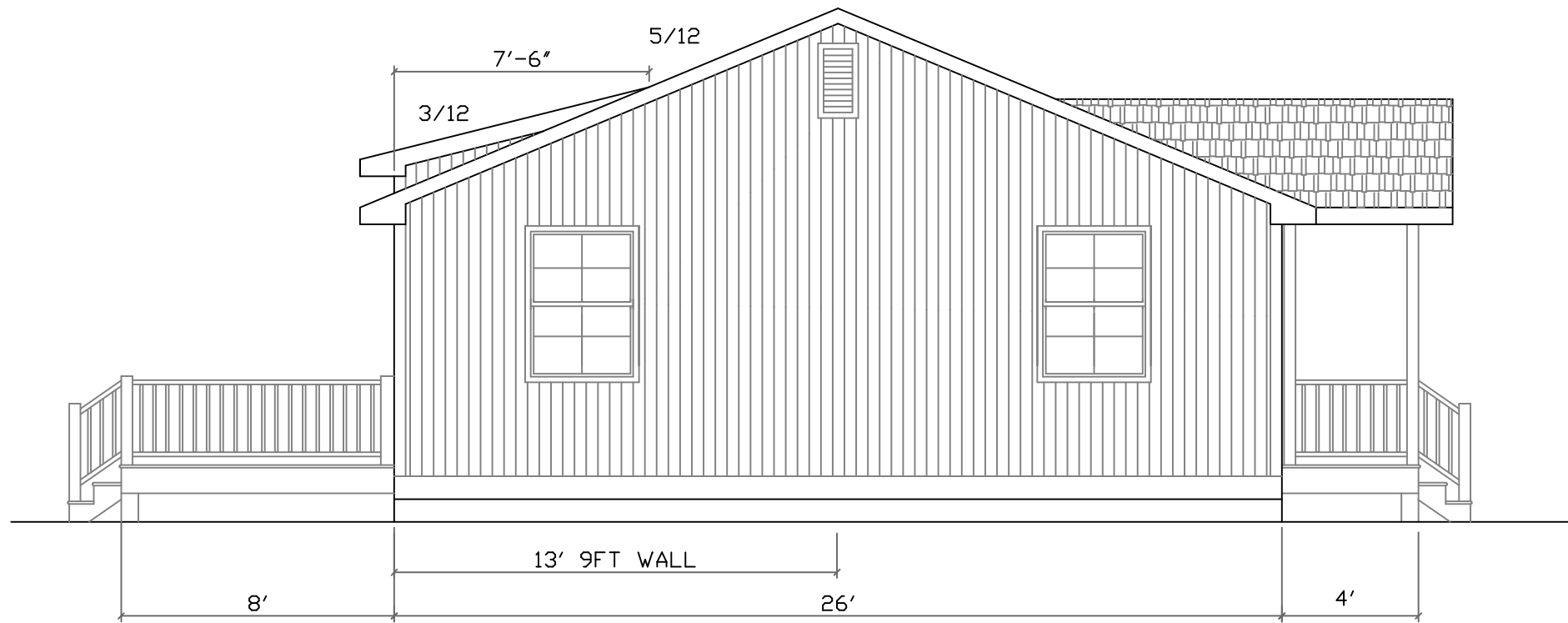
LEFT ELEVATION
